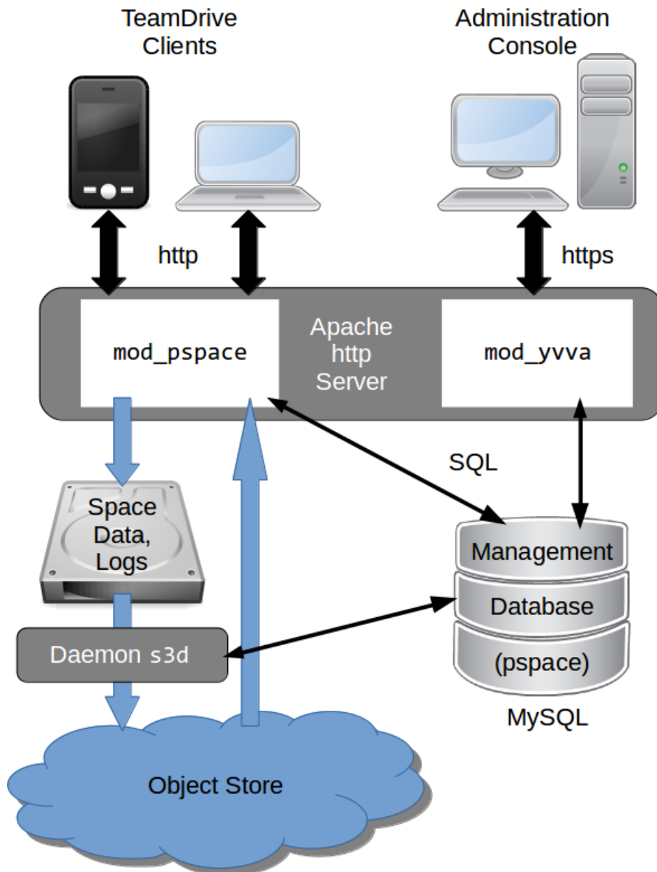
Fig. 4.2: TeamDrive Hosting Service using an object store
