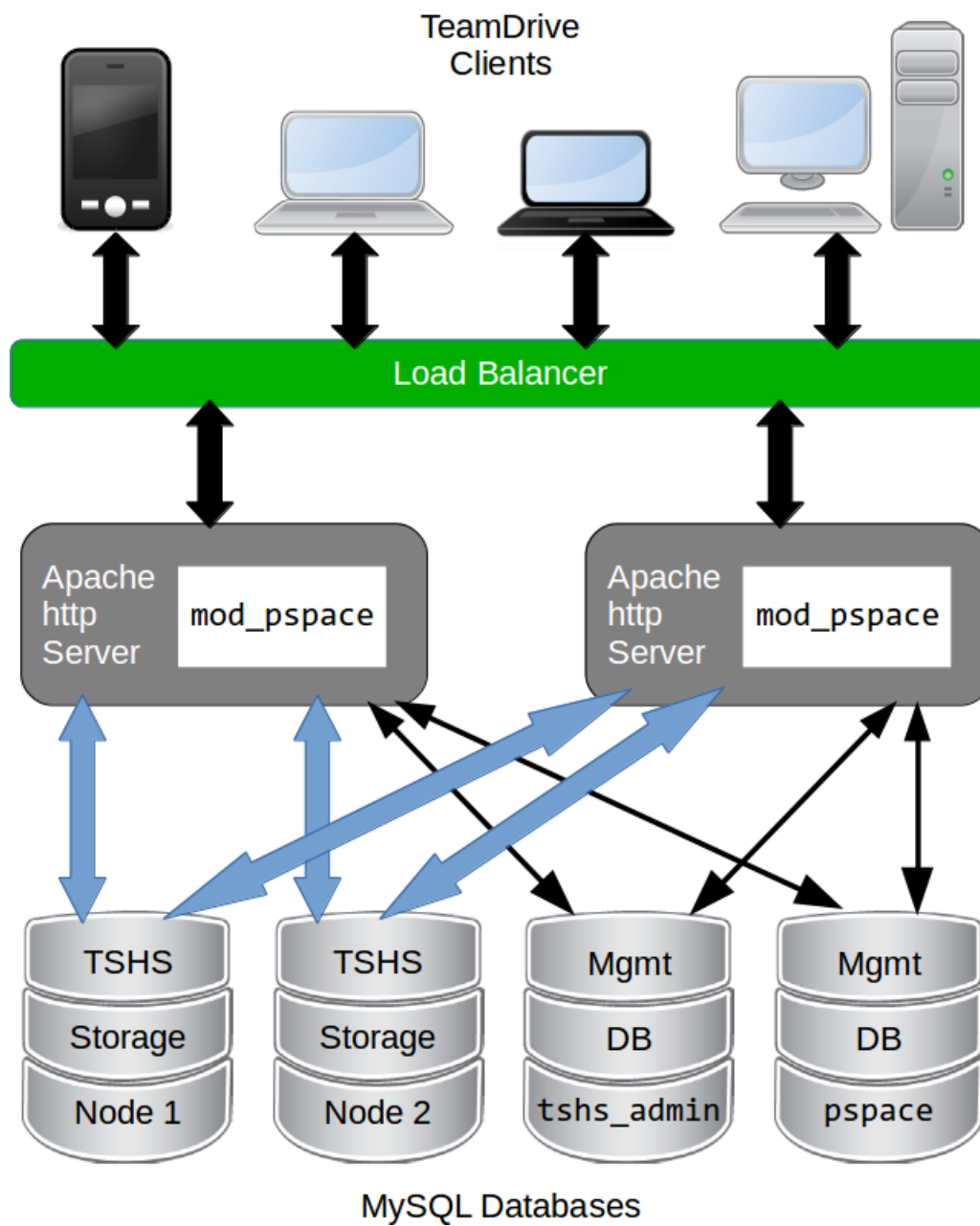
Figure 7.1: TeamDrive Scalable Hosting Storage (TSHS)
