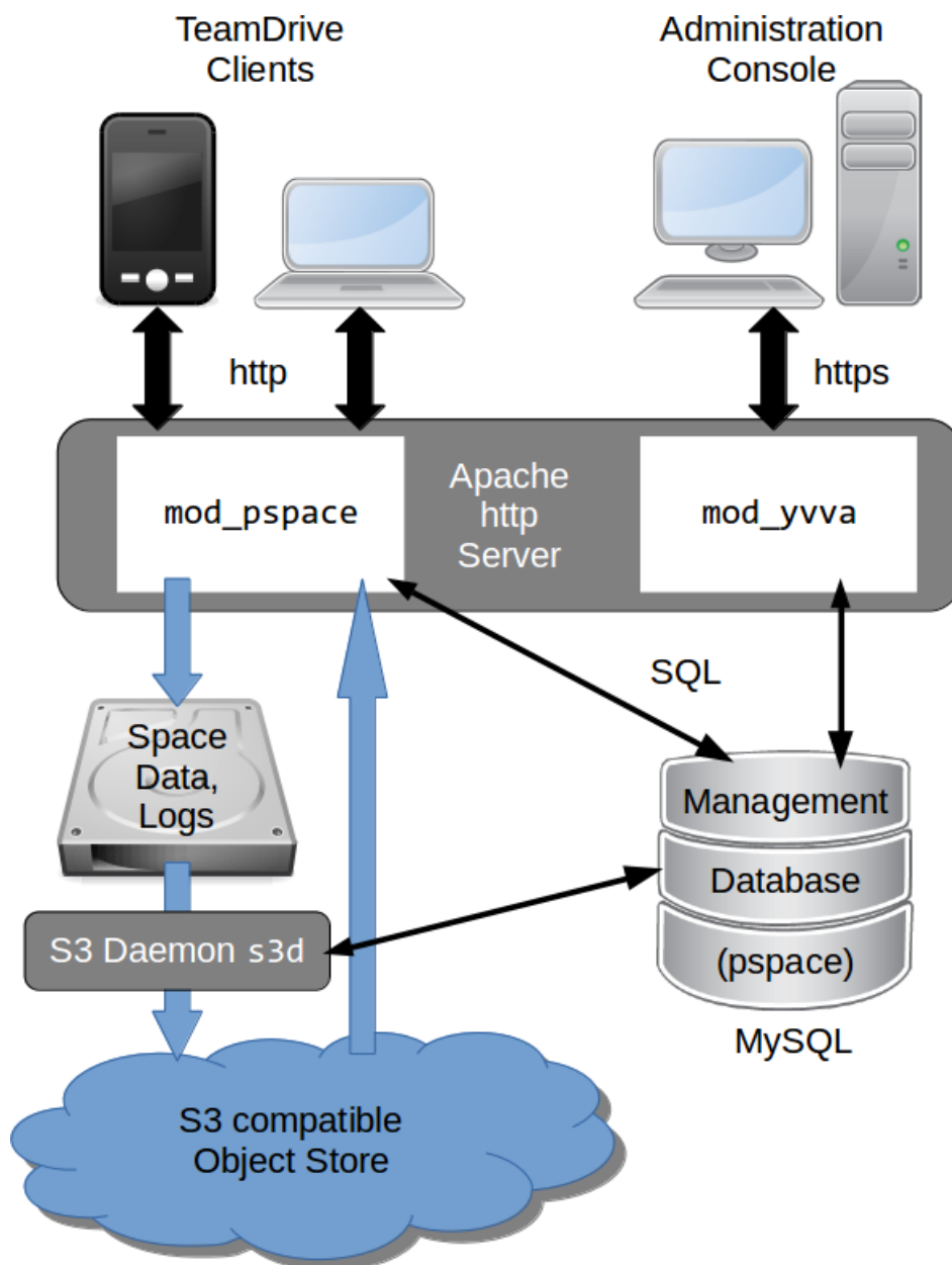
Figure 6.1: TeamDrive Hosting Service using an S3-compatible object store
