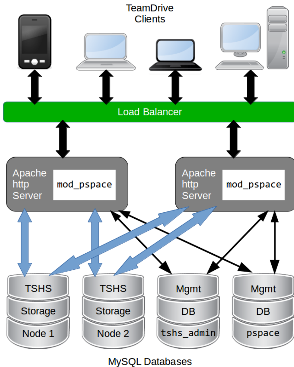
Fig. 9.1: TeamDrive Scalable Hosting Storage (TSHS)
